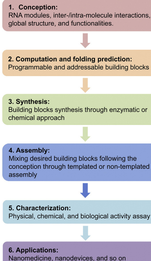
Fig. 1. Approaches to RNA nanotechnology. The construction of RNA nanoparticles starts from a conception design to define the desired properties of the nanoparticles. The RNA structure and folding of building blocks are then computed. After monomeric RNA building block synthesis, the RNA nanoparticles can be assembled following the designed conception. The resulting RNA nanoparticles can be characterized by gel electrophoresis, atomic force microscopy and electron microscopy. After thorough evaluation, the RNA nanoparticles can be used for various applications in vitro and in vivo [29]. This figure was adapted and modified from ref. [29] with permission.
